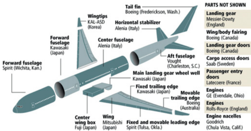
Figure 1 Boeing 787 Dreamliner
