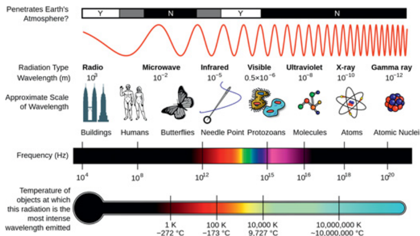
Figure 5 Milton spectrum of radiation wavelengths, frequencies, and black body emission temperatures. Wavelengths relate to electromagnetic radiation from gamma rays to radio waves in the graphic. Example sources or events for each wavelength category demonstrate their natural and technological uses and impacts. The spectrum also indicates the blackbody temperatures at which distinct wavelengths peak, demonstrating the theoretical temperatures at which things emit radiation.
