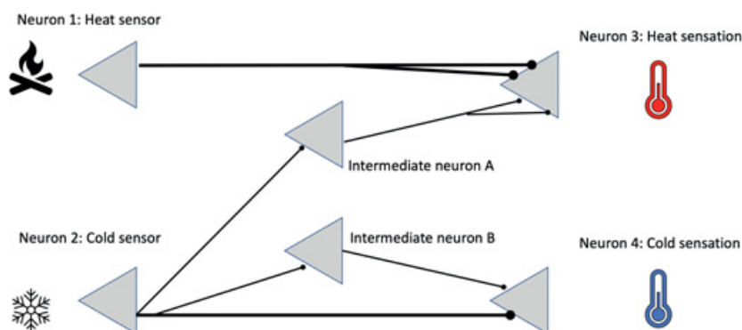
Figure 11 Simplified illustration of McCulloch and Pitts' hypothetical network explaining the heat illusion. When neuron 1 senses heat (ON), it sends a signal to neuron 3, eliciting the sensation of heat. When neuron 2 senses a chilly input and fires once, it sends a signal to intermediary neuron A, which activates neuron 3 and elicits an illusory sensation of heat. If neuron 2 fires twice, it sends a signal to intermediary neuron B, which turns off intermediary neuron A and activates neuron 4, eliciting a cold sensation.
