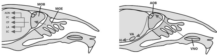
Figure 4 Olfactory and Pheromone Pathways. Distinct anatomical positioning between the Main Olfactory Epithelium (MOE) and the Vomeronasal Organ (VNO) in rodents. In addition, there are significant differences in the genes that express odor and pheromone receptors.
