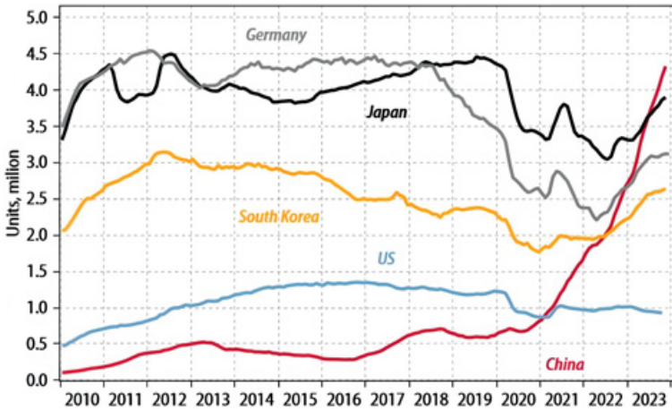
Figure 7 China has become an auto export powerhouse
