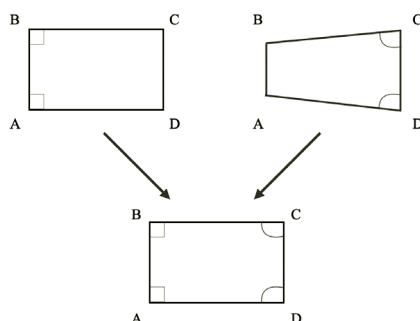
Figure 2 Blending analysis of Saccheri's quadrilateral
