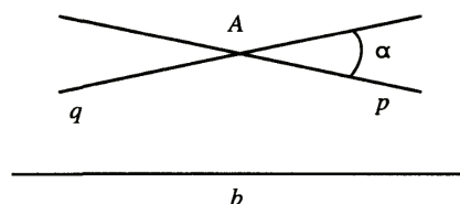
Figure 3 Saccheri's blend, in which, through a point outside a line, there is an infinity of parallel lines
